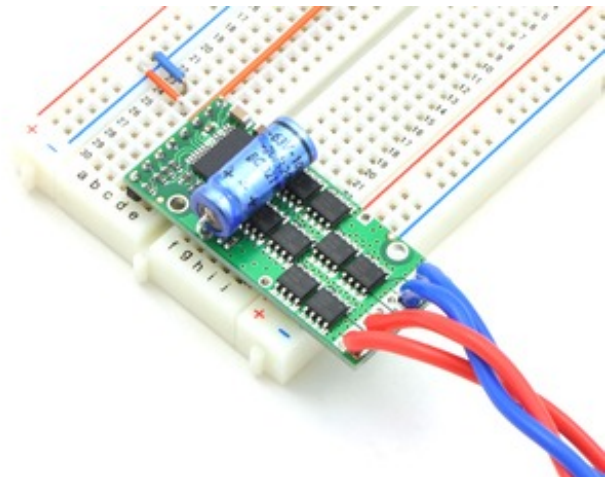
Pololu high-power motor driver in a breadboard.
