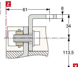
CVS400/630
