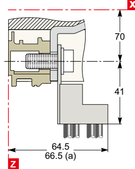
CVS100 to 250
