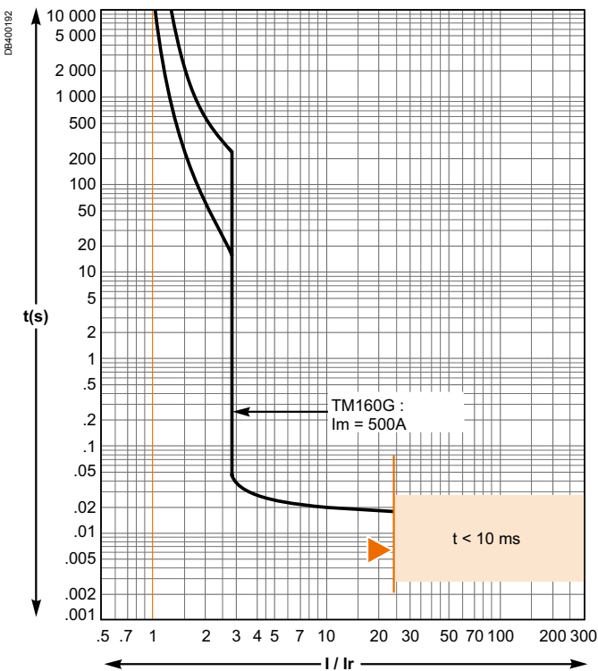
TM160G
