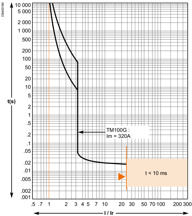
TM100G
