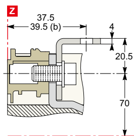
CVS100 to 250
