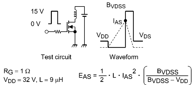
Fig. 9.16 Test Circuit/Waveform
