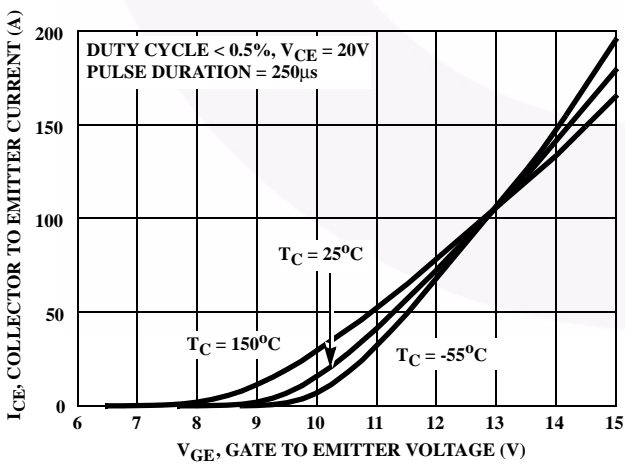
FIGURE 13. TRANSFER CHARACTERISTIC
