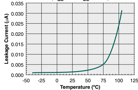
Leakage Current vs. Temperature ( V_{GS}=-5V, V_{DS}=250V )
