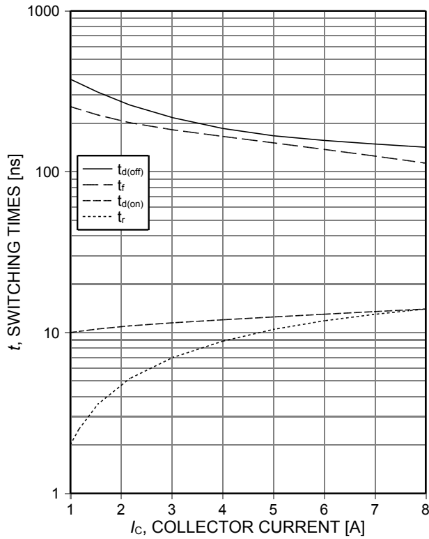
Figure 9. Typical switching times as a function of collector current (inductive load, T_{vj}=175^{\circ}\text{C} , V_{CE}=400\text{V} , V_{GE}=15/0\text{V} , r_G=43\Omega , Dynamic test circuit in Figure E)
