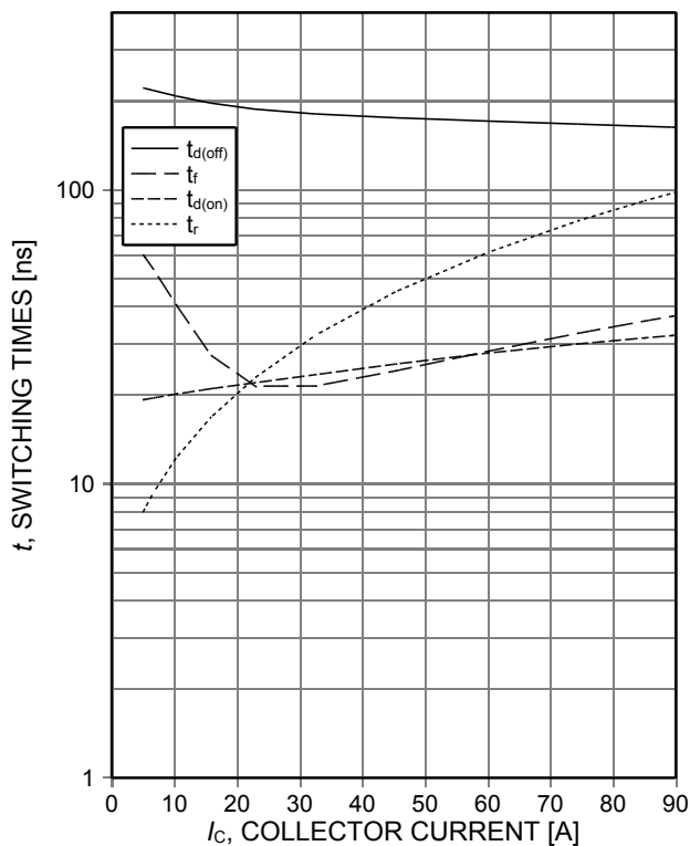
Figure 7. Typical switching times as a function of collector current (inductive load, T_{vj}=150^\circ\text{C} , V_{CE}=400\text{V} , V_{GE}=0/15\text{V} , R_G=22\Omega , Dynamic test circuit in Figure E)
