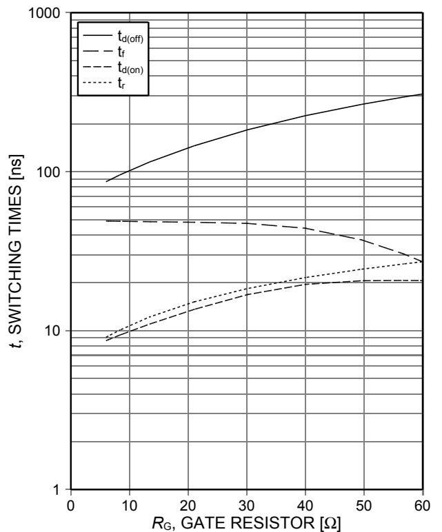
Figure 8. Typical switching times as a function of gate resistor (inductive load, T_{vj}=150^\circ\text{C} , V_{CE}=400\text{V} , V_{GE}=0/15\text{V} , I_c=20\text{A} , Dynamic test circuit in Figure E)
