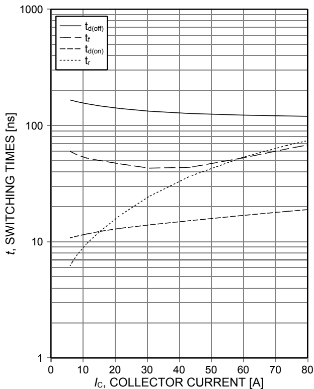
Figure 7. Typical switching times as a function of collector current (inductive load, T_{vj}=150^\circ\text{C} , V_{CE}=400\text{V} , V_{GE}=0/15\text{V} , R_G=20\Omega , Dynamic test circuit in Figure E)
