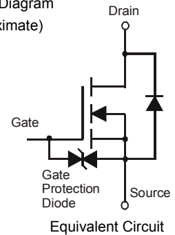
Equivalent Circuit
