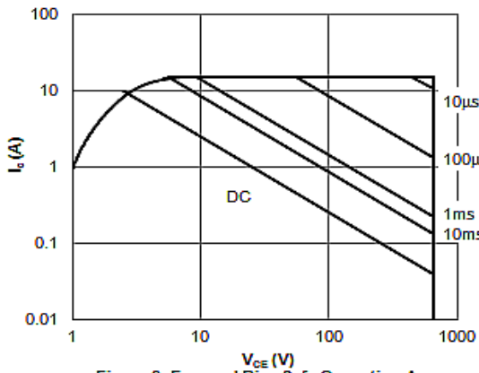
Figure 9: Forward Bias Safe Operating Area ( T_C=25^\circ\text{C} , V_{EE}=15\text{V} )
