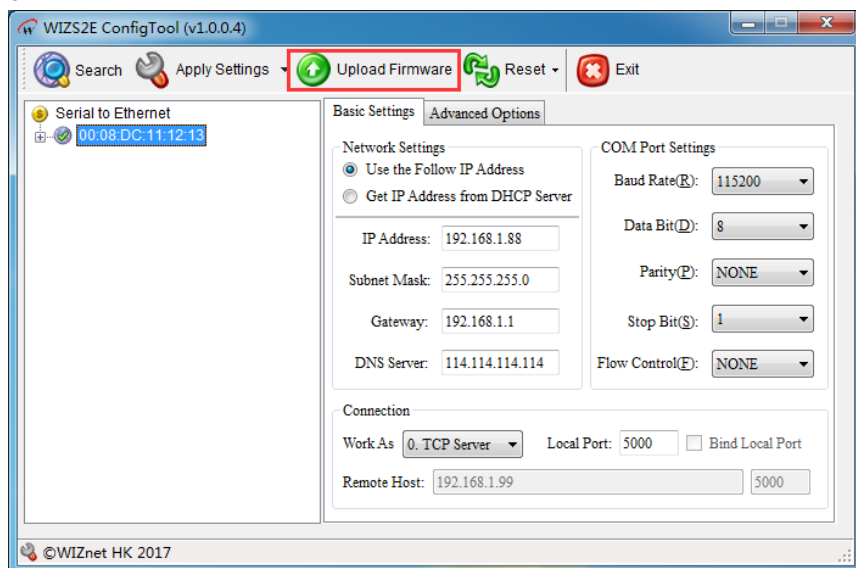
Figure 8-1 W7500S2E-R1 firmware upgrade through ConfigTool
