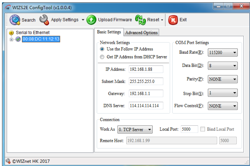
Figure 4-2 WIZS2E ConfigTool search result
