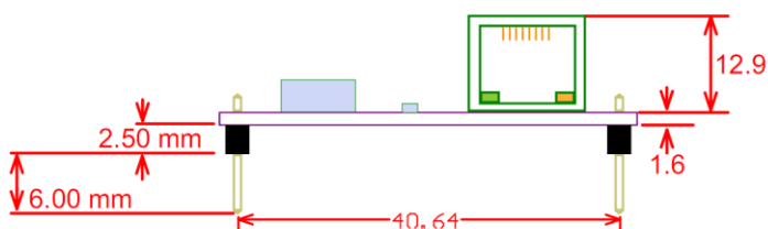
Figure 1-2 W7500S2E-R1 dimensions side view
