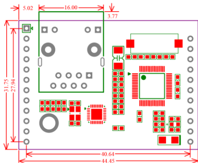
Figure 1-1 W7500S2E-R1 dimensions top view
