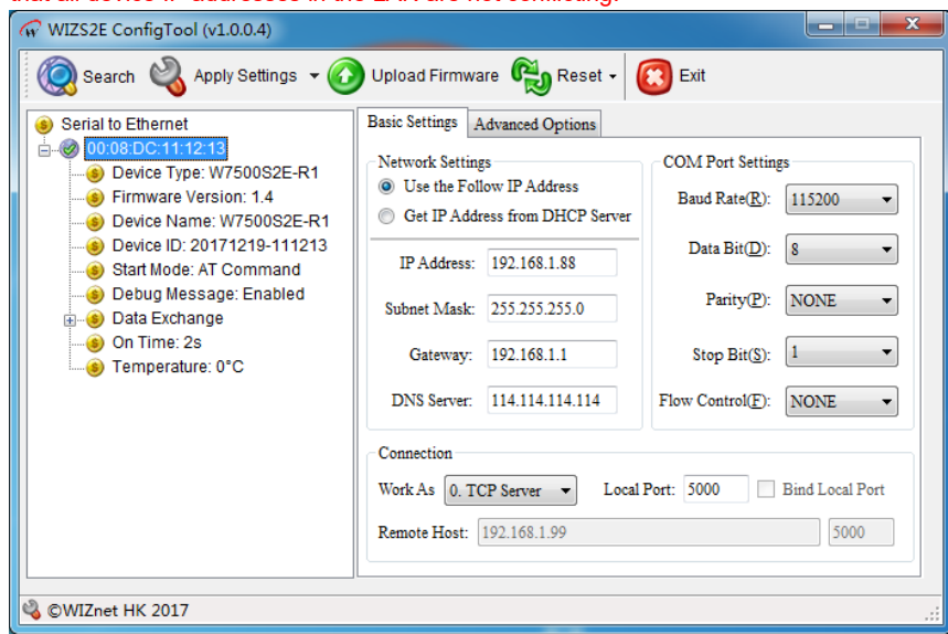
Figure 5-1 WIZS2E ConfigTool basic settings interface
