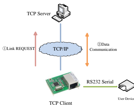
Figure 3-2 TCP client mode diagram
