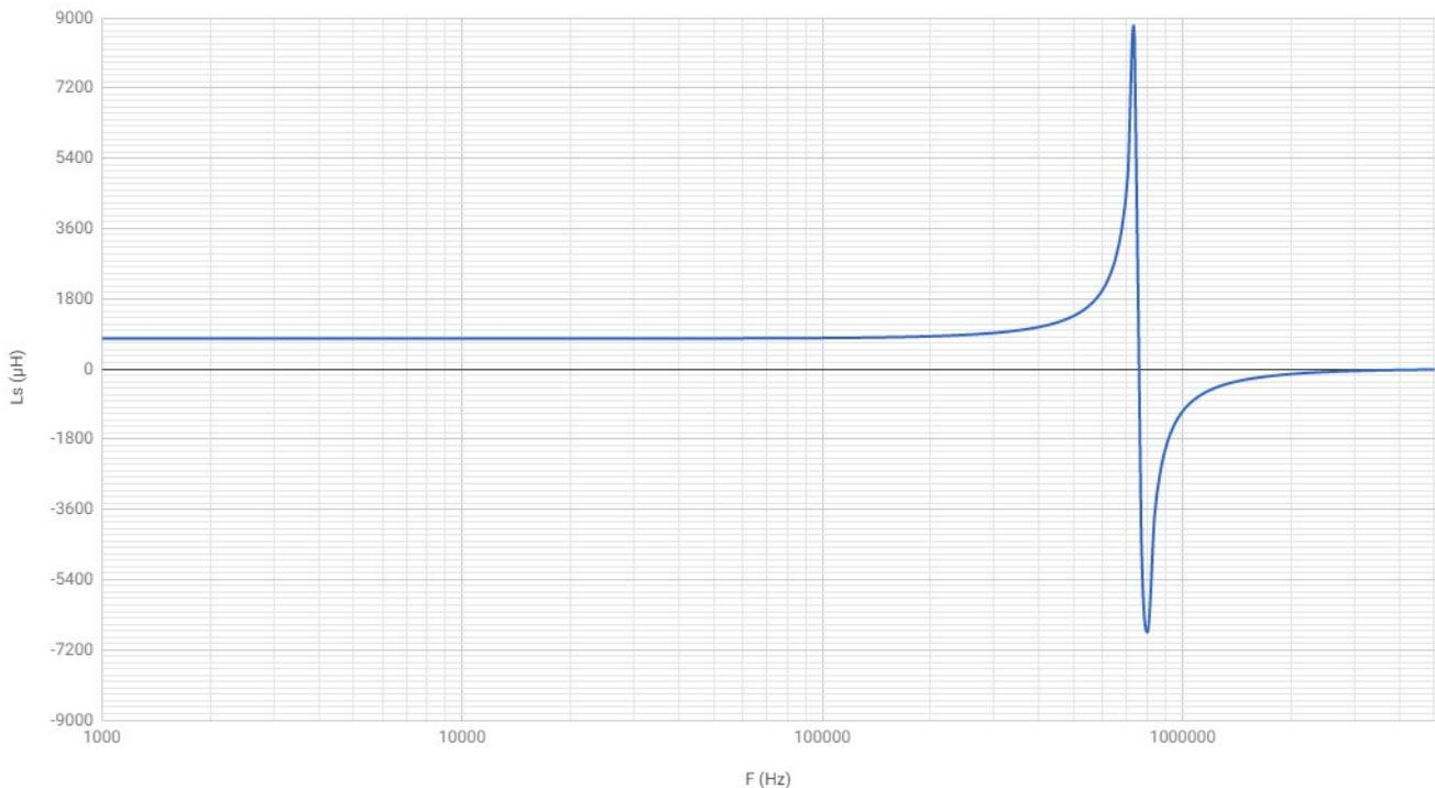
Inductance
