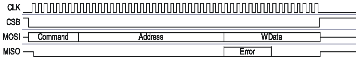
Figure 3: CSPI Register Write Cycle
