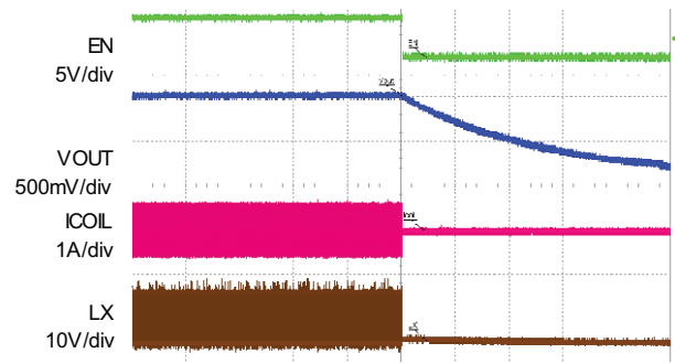
Fig. 14 - Shut-Down, I_{OUT} = 0 \text{ A} Time = 200 \text{ ms}/\text{div}
