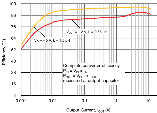
Fig. 10 - SiC437 Efficiency vs. Output Current (VIN = 12 V, fsw = 500 kHz, Power Saving Mode)
