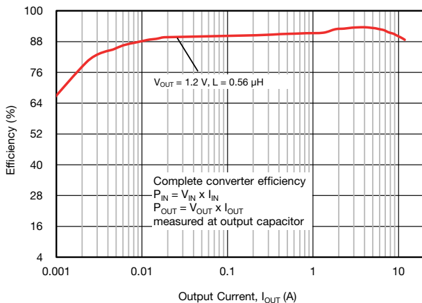
Fig. 12 - SiC437 Efficiency vs. Output Current (VIN = 5 V, fsw = 500 kHz, Power Saving Mode)
