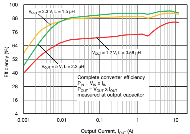
Fig. 15 - SiC437 Efficiency vs. Output Current (VIN = 24 V, fsw = 500 kHz, Power Saving Mode)
