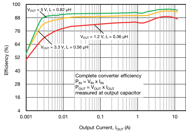
Fig. 13 - SiC437 Efficiency vs. Output Current (VIN = 12 V, fsw = 1 MHz, Power Saving Mode)
