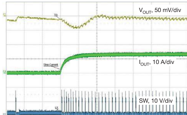
Fig. 31 - Load Step, 0.1 A to 12 A, 1 A/ \mu\text{s} , t = 10\ \mu\text{s}/\text{div} Skip Mode Enabled
