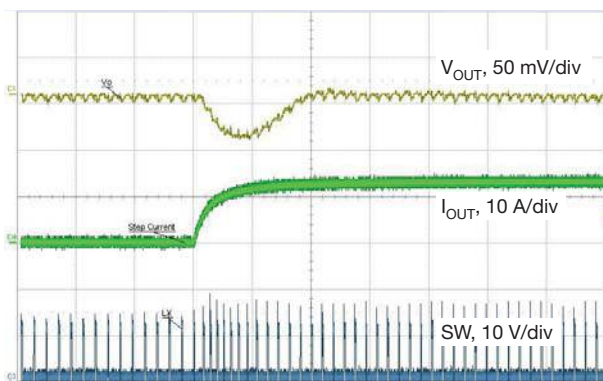
Fig. 32 - Load Step, 0.1 A to 12 A, 1 A/ \mu\text{s} , t = 10\ \mu\text{s}/\text{div} Forced Continuous Conduction Mode
