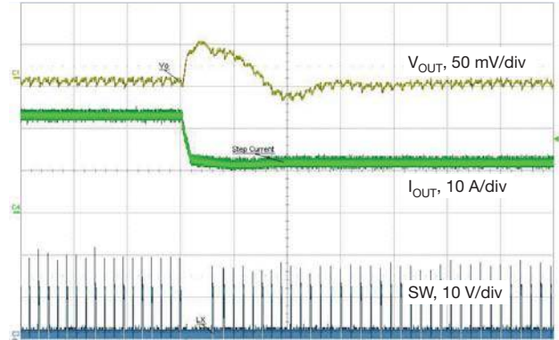
Fig. 33 - Load Release, 24 A to 12 A, 1 A/ \mu\text{s} , t = 10\ \mu\text{s}/\text{div}
