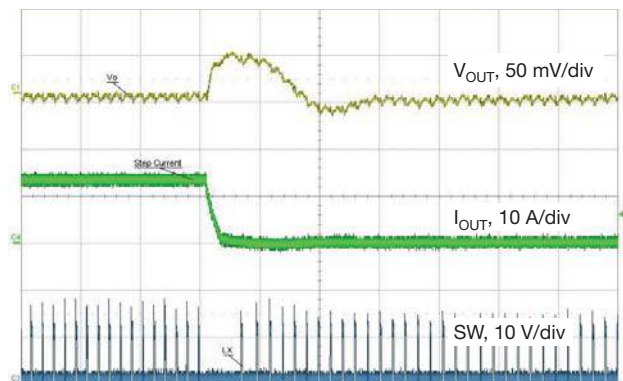
Fig. 35 - Load Release, 12 A to 0.1 A, 1 A/ \mu\text{s} , t = 20\ \mu\text{s}/\text{div} Forced Continuous Conduction Mode
