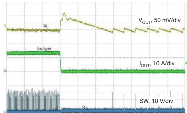
Fig. 34 - Load Release, 12 A to 0.1 A, 1 A/ \mu\text{s} , t = 50\ \mu\text{s}/\text{div} Skip Mode Enabled
