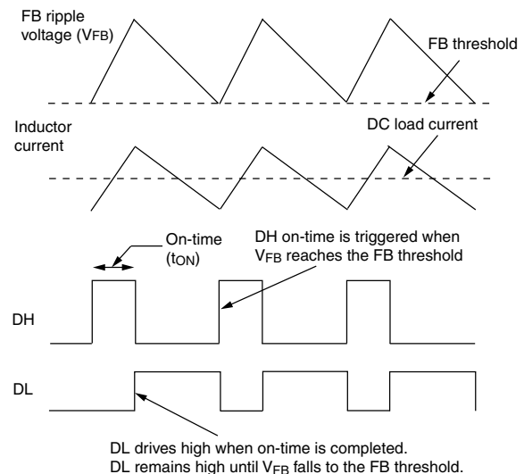
Fig. 26 - Forced Continuous Mode Operation
