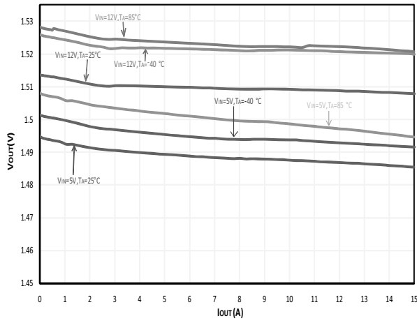
Load Regulation vs. Temperature - FCM (V DD = 5 V, V OUT T = 1.5 V, SiC401B)
