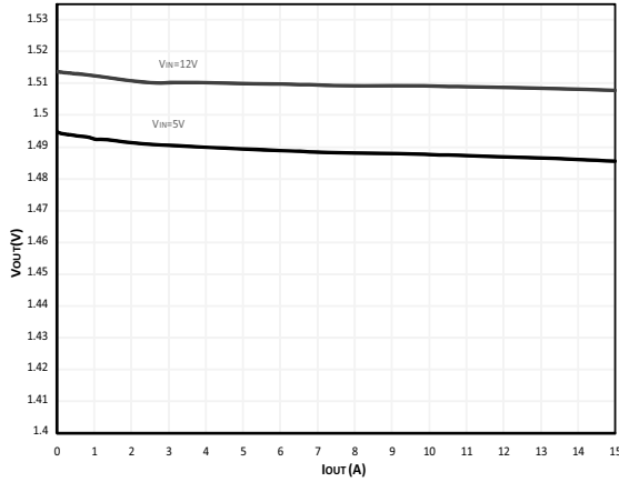
Load Regulation - FCM (V DD = 5 V, V OUT = 1.5 V, SiC401B)
