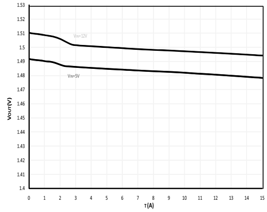
Load Regulation - FCM (V DD = 3.3 V, V OUT = 1.5 V, SiC401B)
