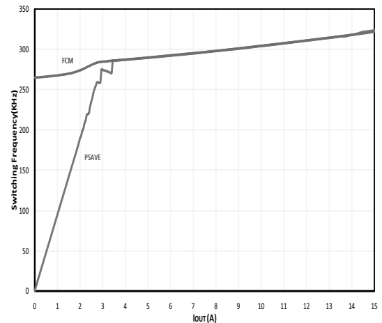
Switching Frequency - P-Save vs. FCM (V DD = 3.3 V, V OUT = 1.5 V, V IN = 12 V, SiC401B)
