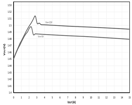
Load Regulation - P-Save (V DD = 3.3 V, V OUT = 1.5 V, SiC401B)
