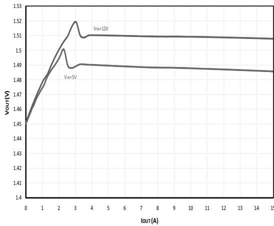
Load Regulation - P-Save (V DD = 5 V, V OUT = 1.5 V, SiC401B)
