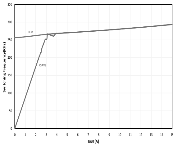
Switching Frequency - P-Save Mode vs. FCM (V DD = 5 V, V OUT = 1.5 V, V IN = 12 V, SiC401B)
