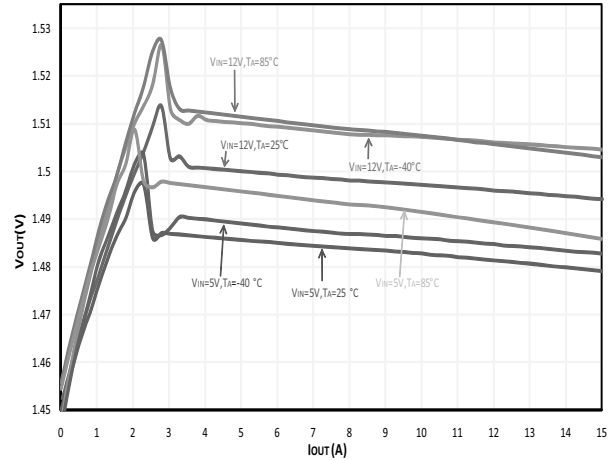
Load Regulation vs. Temperature - P-Save (V DD = 3.3 V, V OUT T = 1.5 V, SiC401B)
