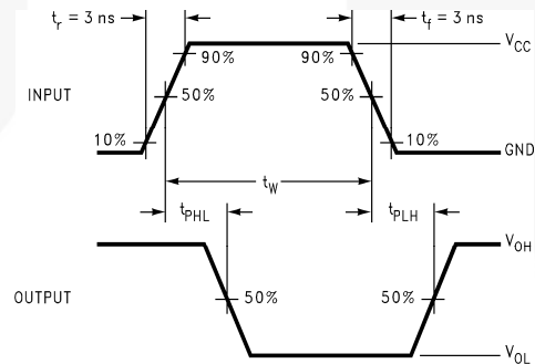
Figure 6. AC Waveforms
