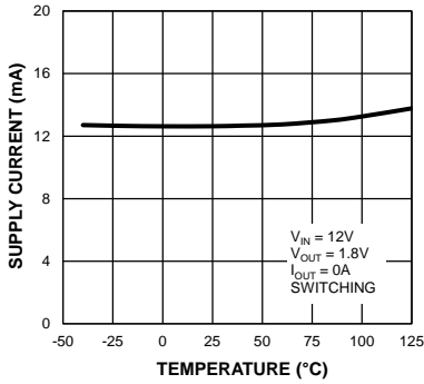
V IN Operating Supply Current vs. Temperature
