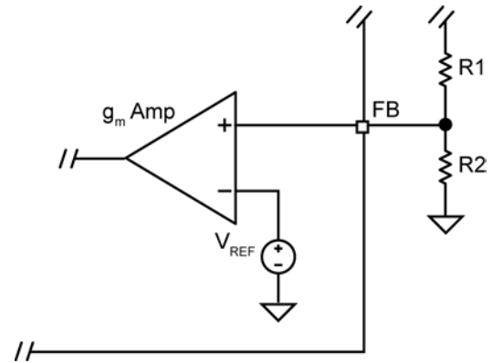
Figure 8. Voltage-Divider Configuration
