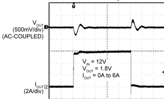
Transient Response
