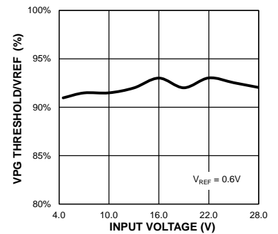
PG/ V_{REF} Ratio vs. Input Voltage
