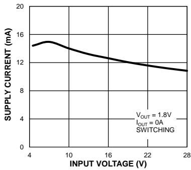
V_{IN} Operating Supply Current vs. Input Voltage
