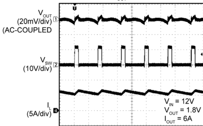
Switching Waveforms
