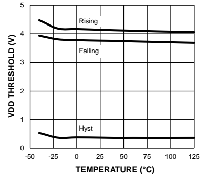
V DD UVLO Threshold vs. Temperature
