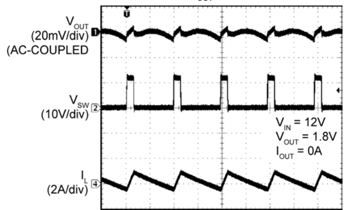
Switching Waveforms
