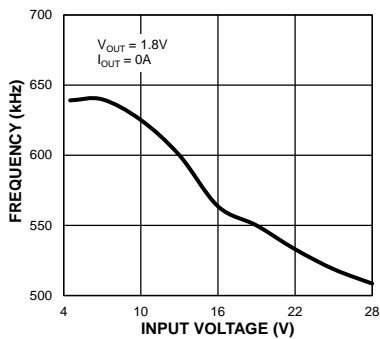
Switching Frequency vs. Input Voltage
