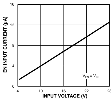
Enable Input Current vs. Input Voltage
