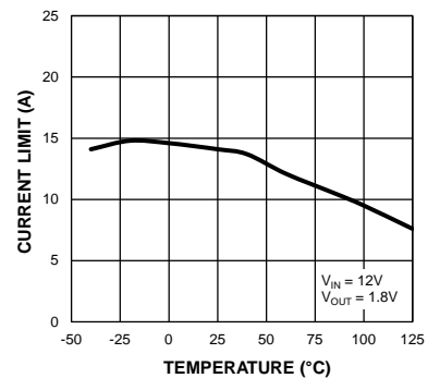
Current Limit vs. Temperature
