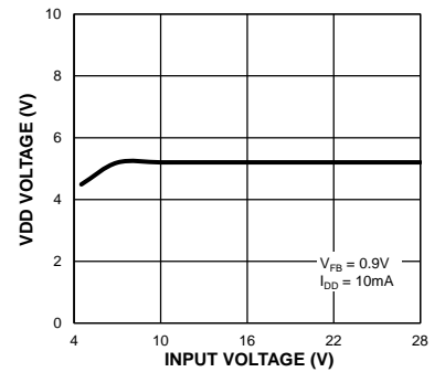
V_{DD} Output Voltage vs. Input Voltage
