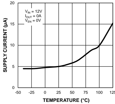
V IN Shutdown Current vs. Temperature
