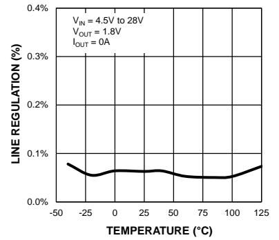
Line Regulation vs. Temperature
