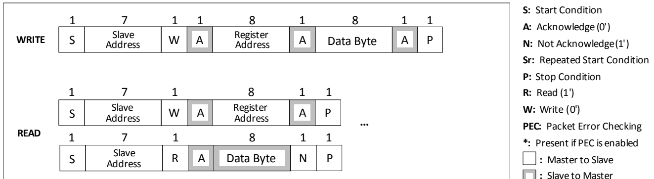
Figure 24: I2C Format
