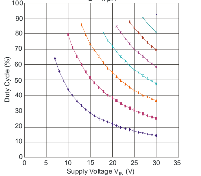
ZXLD1360 Duty Cycle L = 47μH
