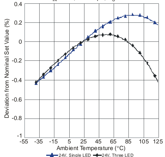
Output Current Change vs. Temperature V IN = 24V, L = 470µH, R S = 0.33Ω
