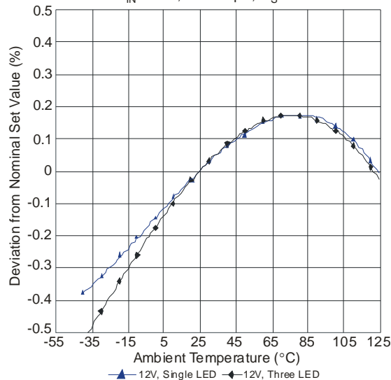
Output Current Change vs. Temperature V IN = 12V, L = 470µH, R S = 0.33Ω
