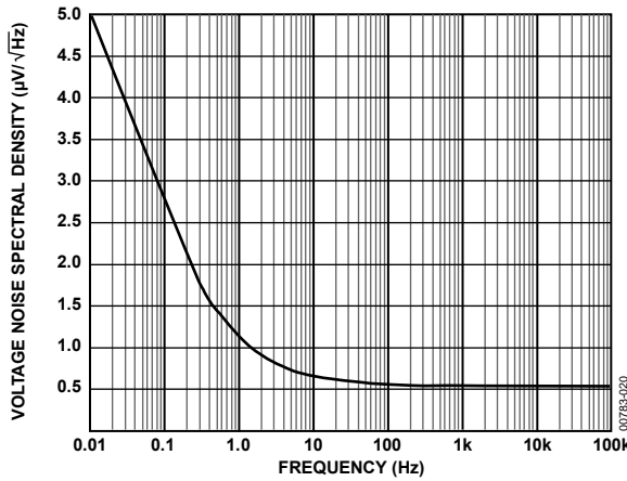
Figure 19. Voltage Noise Spectral Density vs. Frequency
