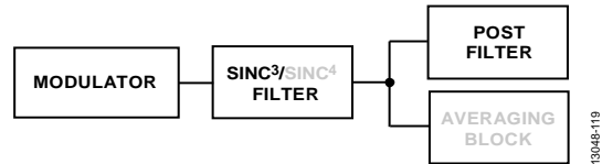
Figure 112. Post Filters
