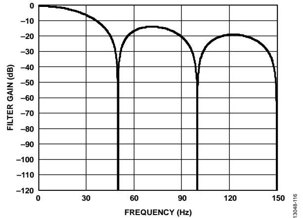
Figure 109. 50 Hz Rejection
