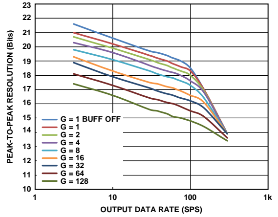
Figure 55. Peak-to-Peak Resolution vs. Output Data Rate, Sinc^3 + Sinc^1 Filter (Mid Power Mode)
