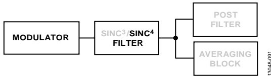
Figure 84. Sinc 4 Filter
