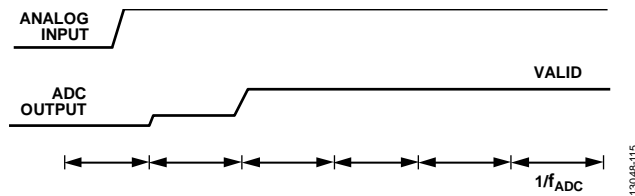
Figure 108. Step Change on the Analog Input, Sinc 3 + Sinc 1 Filter
