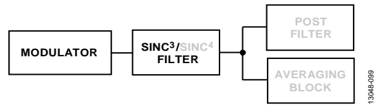
Figure 92. Sinc 3 Filter
