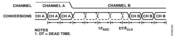
Figure 85. Sinc 4 Channel Change
