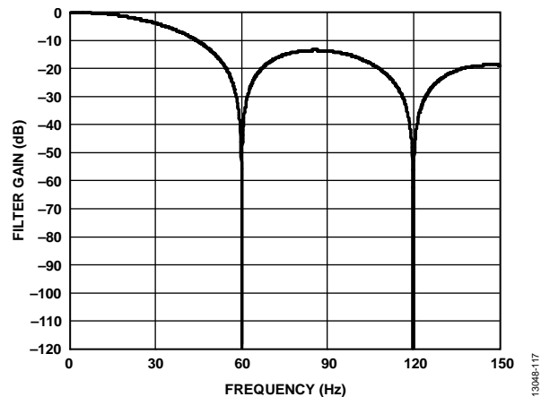
Figure 110. 60 Hz Rejection
