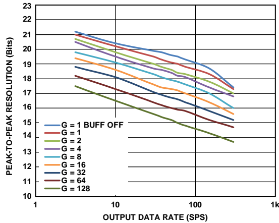
Figure 54. Peak-to-Peak Resolution vs. Output Data Rate, Sinc^4 + Sinc^1 Filter (Mid Power Mode)
