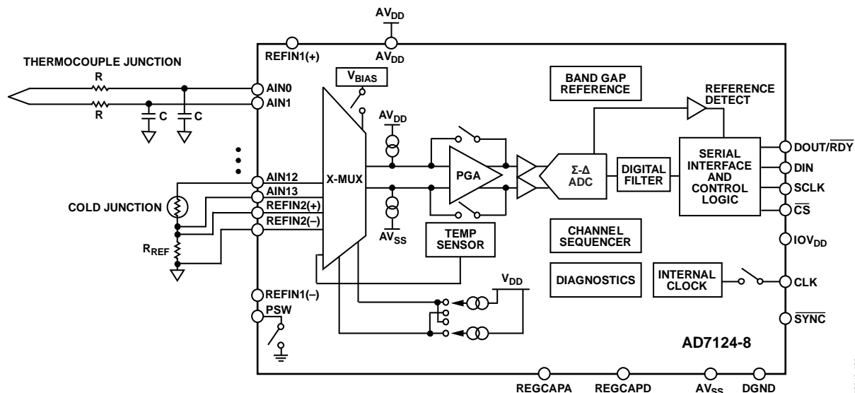
Figure 129. Thermocouple Application
