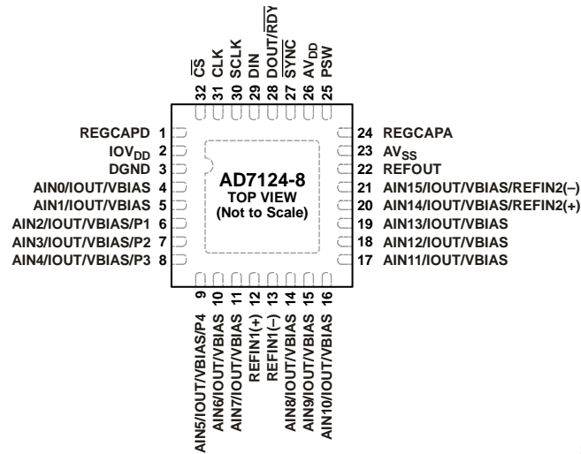
Figure 9. Pin Configuration
