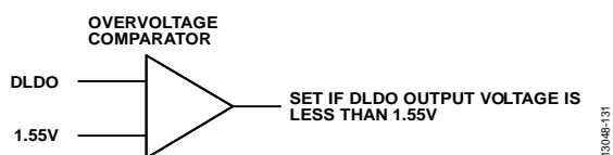
Figure 124. Digital LDO Monitor
