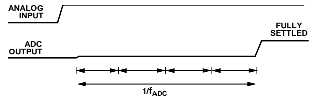
Figure 87. Sinc 4 Zero Latency Operation
