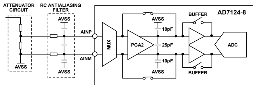
Figure 76. Input Schematic
