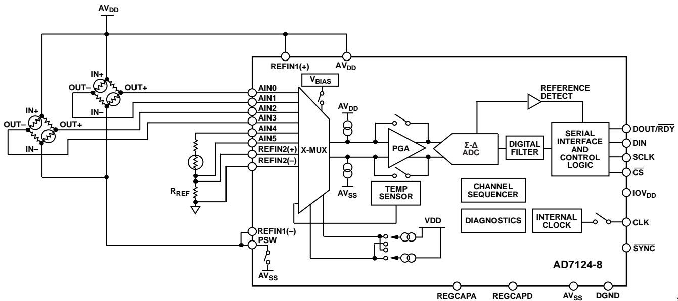
Figure 131. Flowmeter Application
