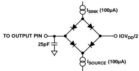
Figure 2. Load Circuit for Timing Characterization
