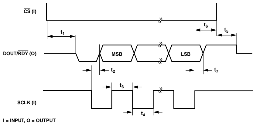
Figure 3. Read Cycle Timing Diagram ( \overline{\text{CS\_EN}} Bit Cleared)
