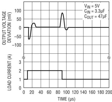
Transient Response
