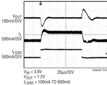
Load Step
