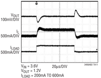
Load Step
