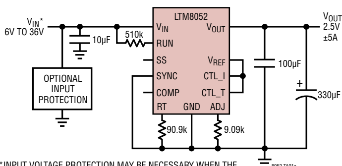
±5A, 2.5V (2-Quadrant) µModule Voltage Regulator
