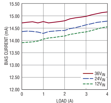
Bias Current vs Load, V_{OUT} = 2.5V
