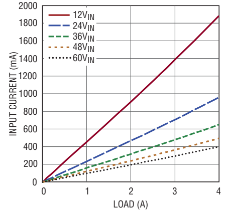
Input Current vs Load, V_{OUT} = 5V
