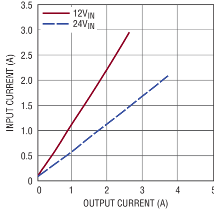
Input Current vs Load Current -12V OUT
