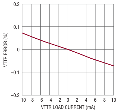
VTR Load Regulation
