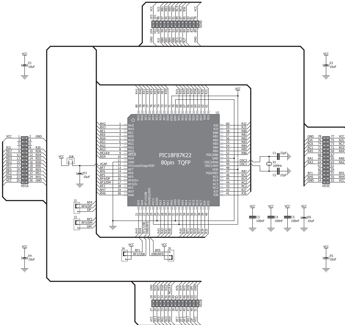
Figure 2: MCU card schematics
