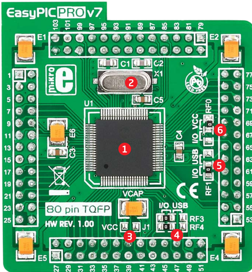
Figure 1: MCU card with PIC18F87K22
