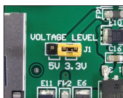
Figure 1-3: J1 in 3.3V position
