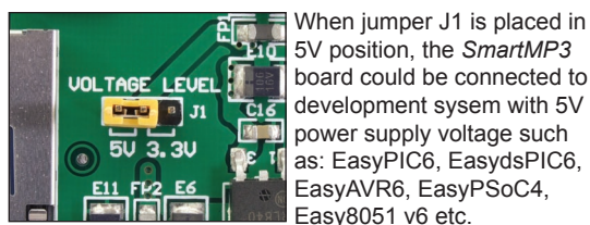
Figure 1-2: J1 in 5V position
