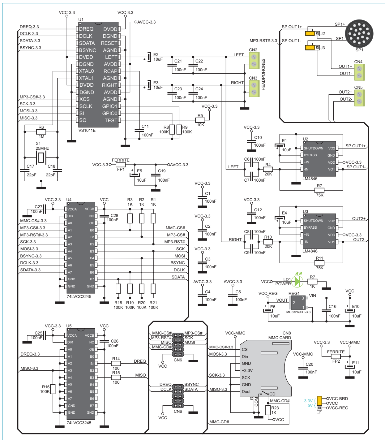
Figure 1-6: SmartMP3 additional board connection schematic
