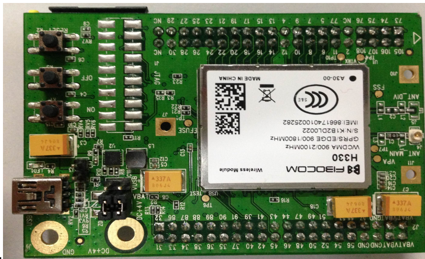
Figure 3-1 ADP-H330 Top View
