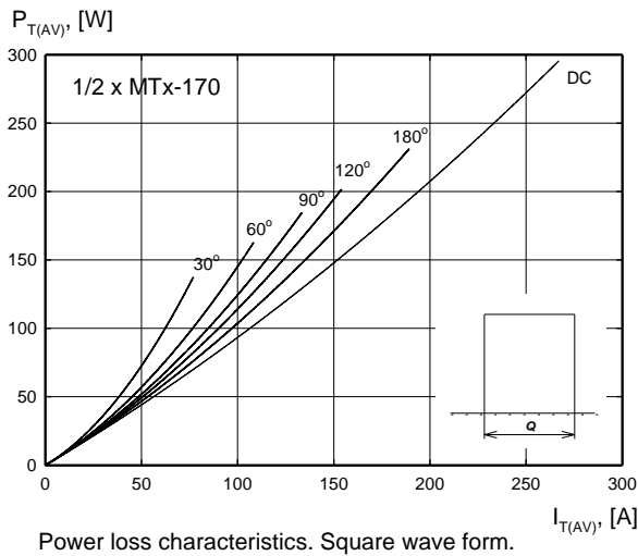
Power loss characteristics. Square wave form.
