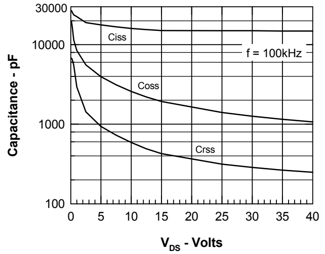
Fig. 8 Capacitance Curves
