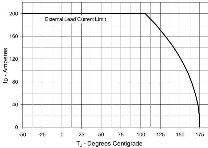
Fig. 5. Maximum Drain Current vs. Case Temperature
