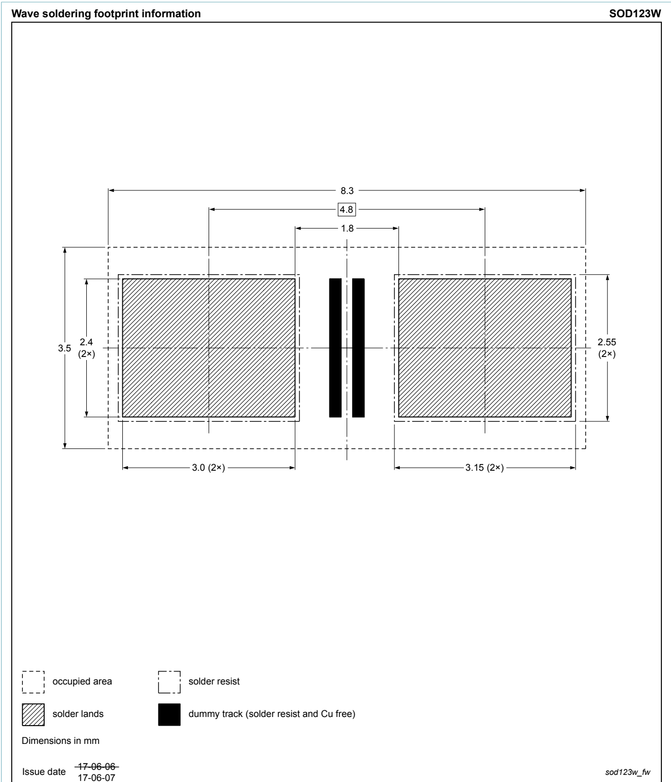
Fig. 17. Wave soldering footprint for CFP3 (SOD123W)
