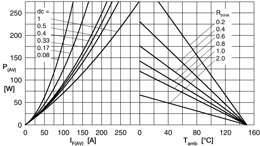
Fig. 4a Power dissipation versus direct output current Fig. 4b and ambient temperature
