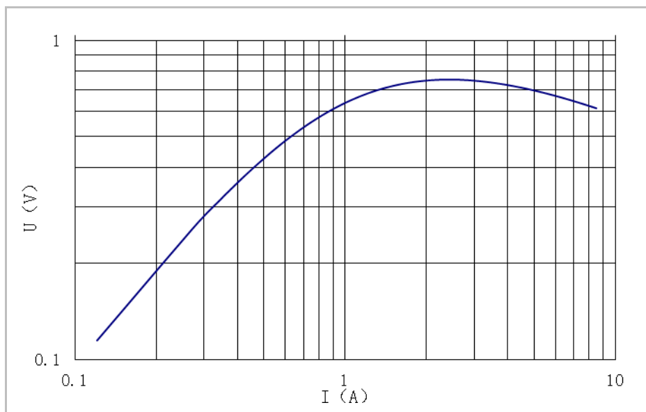
figure 5: V—I curve
