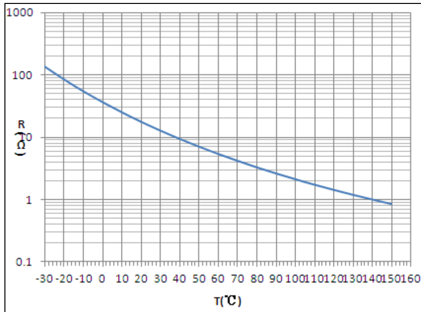
figure 4 R—T curve
