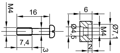
Bottom part of box 8100.8005 and on a screw M4x16
