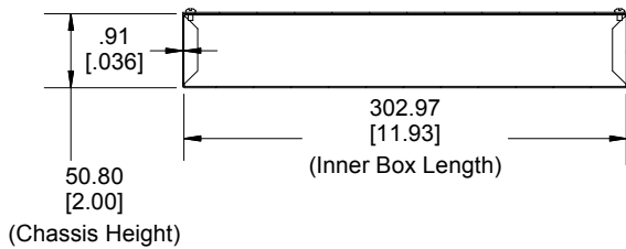
SECTION B-B Side View of Assembly
