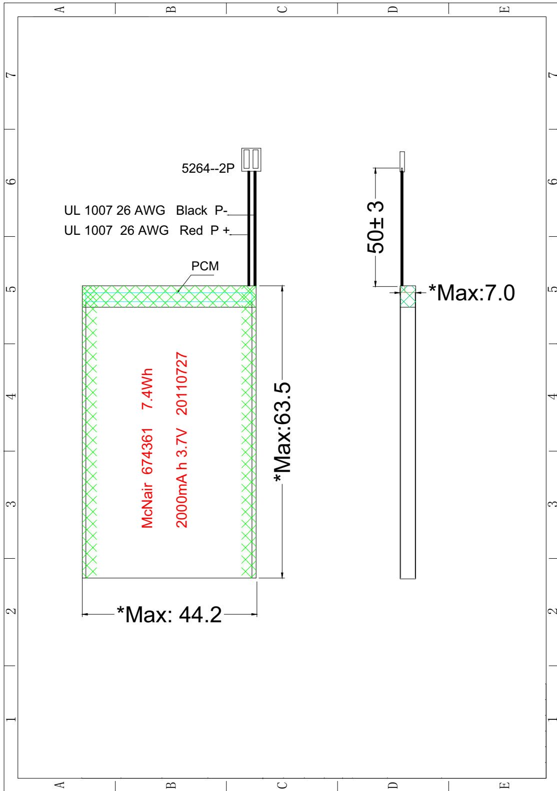
Fig.1 OUTLINE DRAWING
