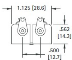
CAT. NO. 1290-79 Solder Lugs
