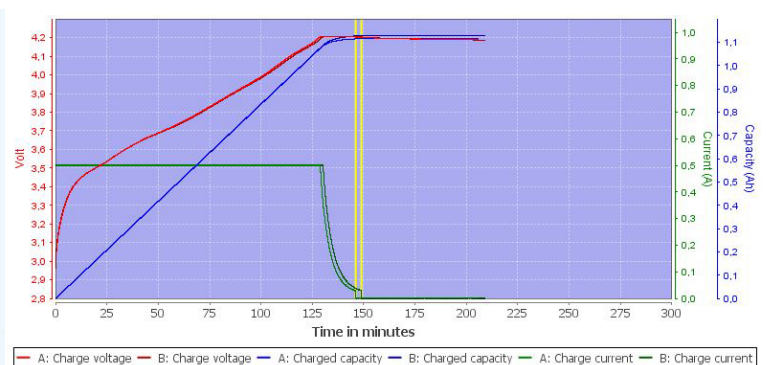
Characteristics of charging the cell ICR18650-300PCM-R
