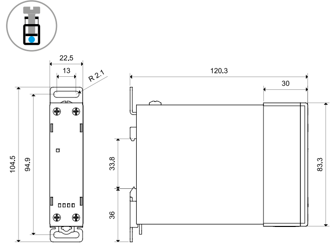
77.11/31 Screw terminal
