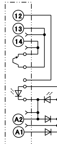
12 V DC Terminal Arrangement/ Internal Connections (Top View)
