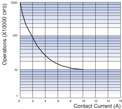
ENDURANCE CURVE
