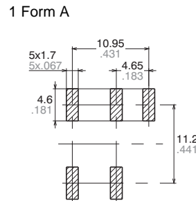
Recommended mounting pad (Top view)
