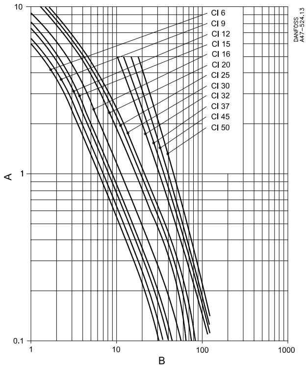
Contactors CI 6/9/12/15, CI 16/20/25/30, CI 37/45/50, load categories AC-3
